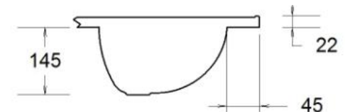
Elevation Through Bowl
